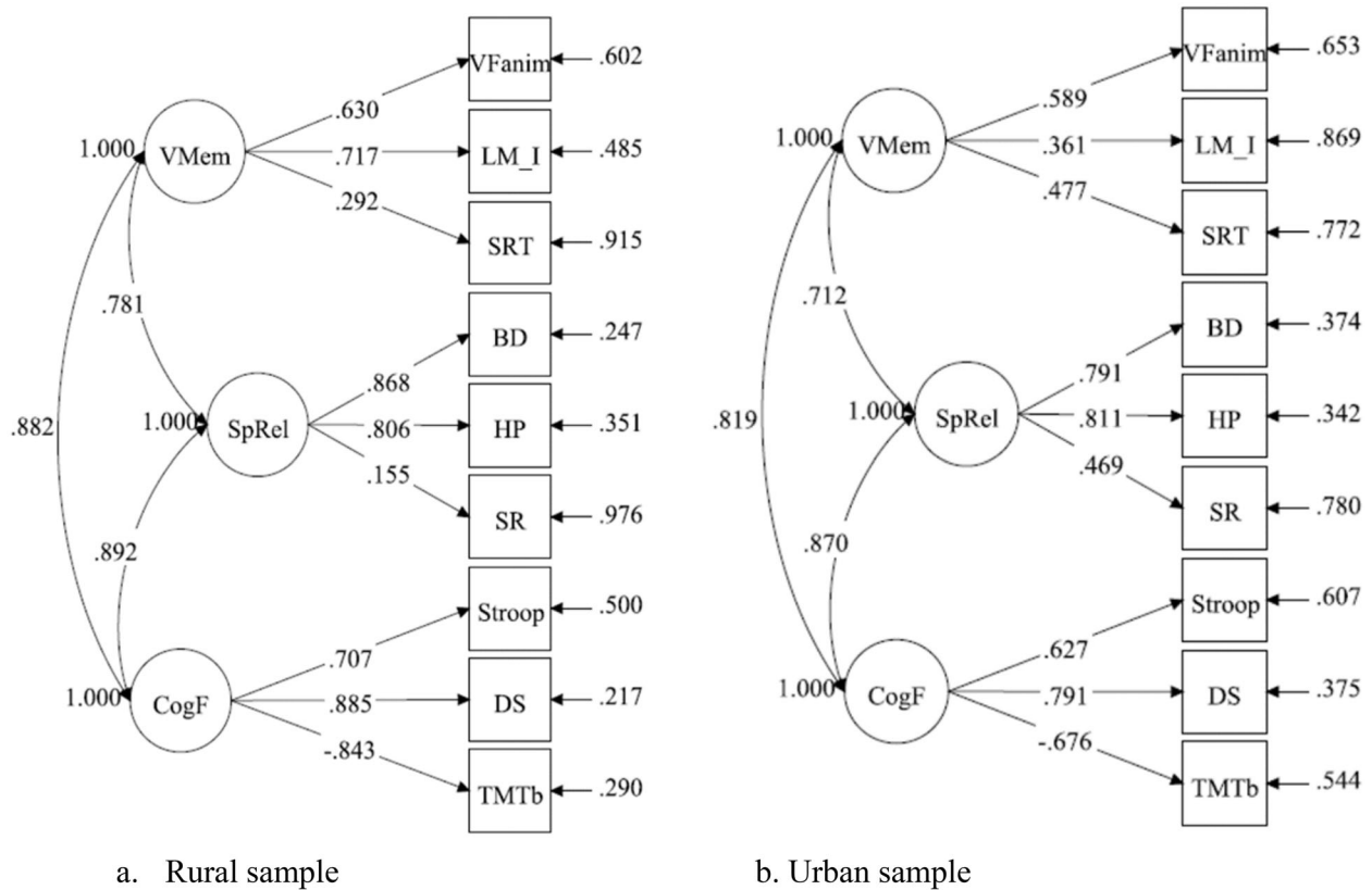
Figure 1. Confirmatory Factorial Analysis (CFA) baseline model with three cognitive latent factors and nine neuropsychological tests. (a) Rural sample. (b) Urban sample. Note. Latent variables: VMem = Verbal memory; SpRel = Spatial relations; CogF = Cognitive flexibility. Neuropsychological tests: VFanim = Verbal fluency animals; LM_I = Logical memory immediate recall; SRT = Selective reminding test total score; BD = Block Design; HP = Hidden Pattern; SR = Spatial relations; Stroop = Stroop Color-word interference; DS = Digit Symbol; TMTb = Trail Making Test b time.
